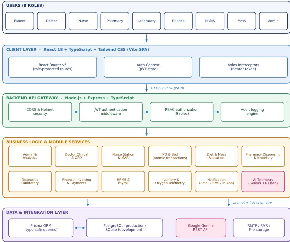
Figure 1 - SHMS layered system architecture
