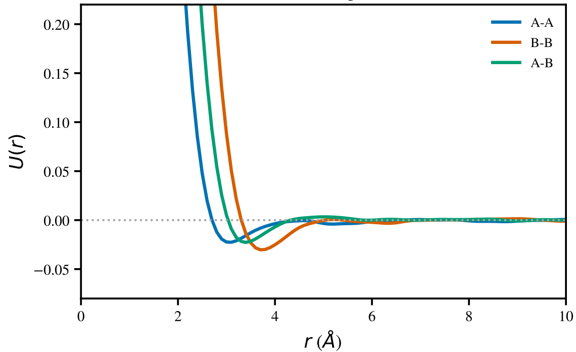
IBI/PMF solute potentials
