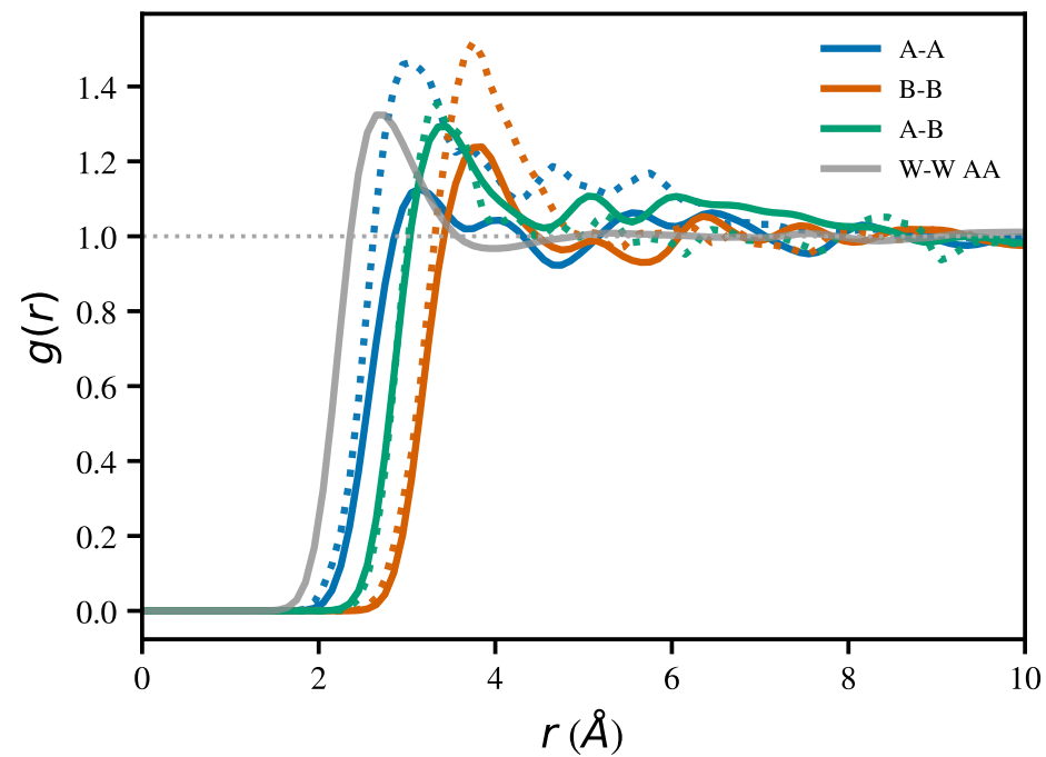
Bulk RDF
