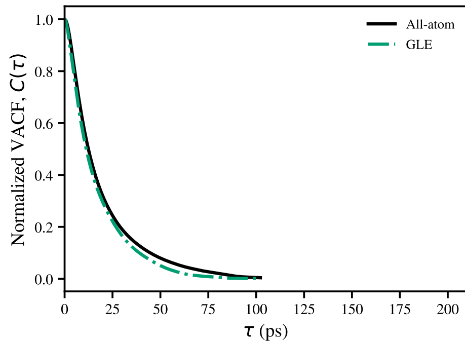
Bulk VACF
