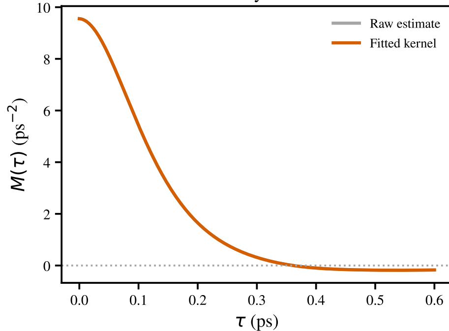
Memory kernel
