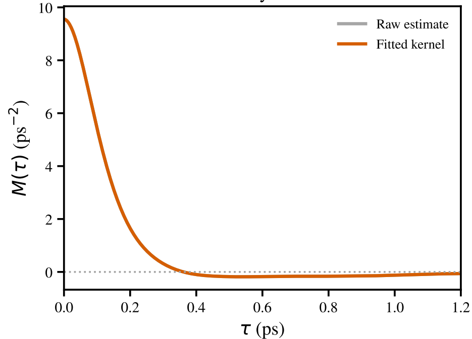
Memory kernel
