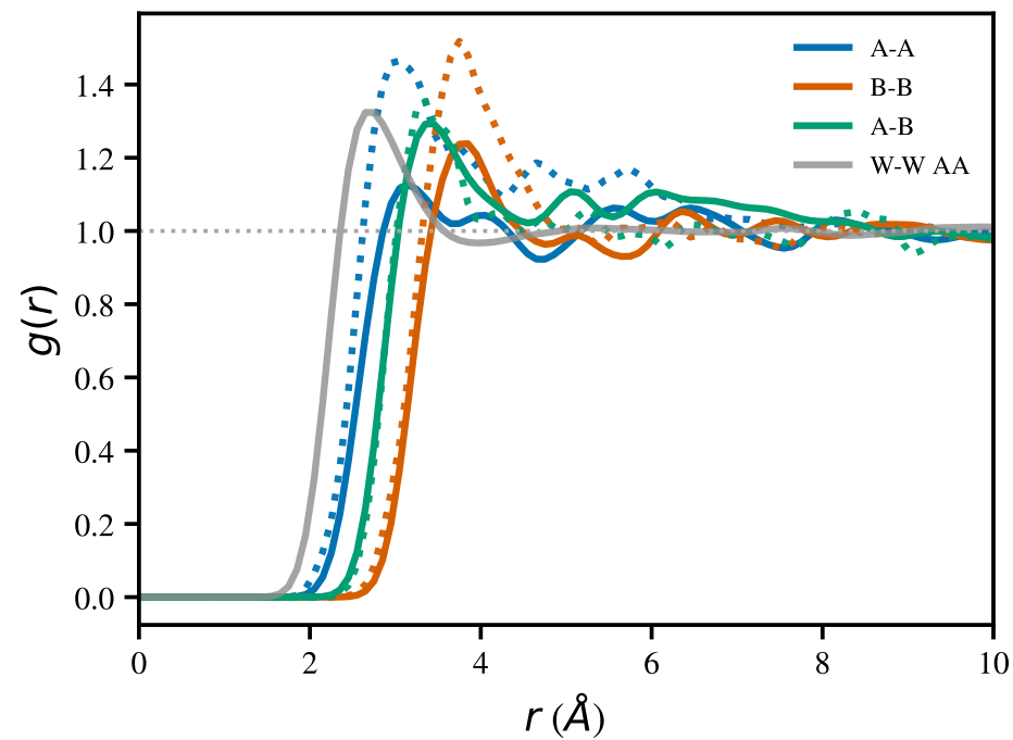
Bulk RDF
