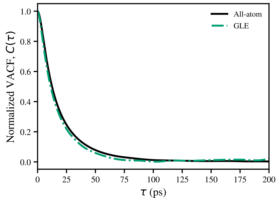
Bulk VACF
