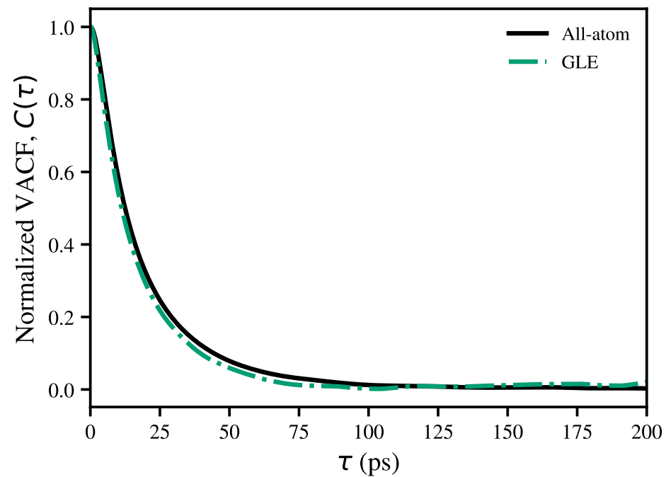
Bulk VACF
