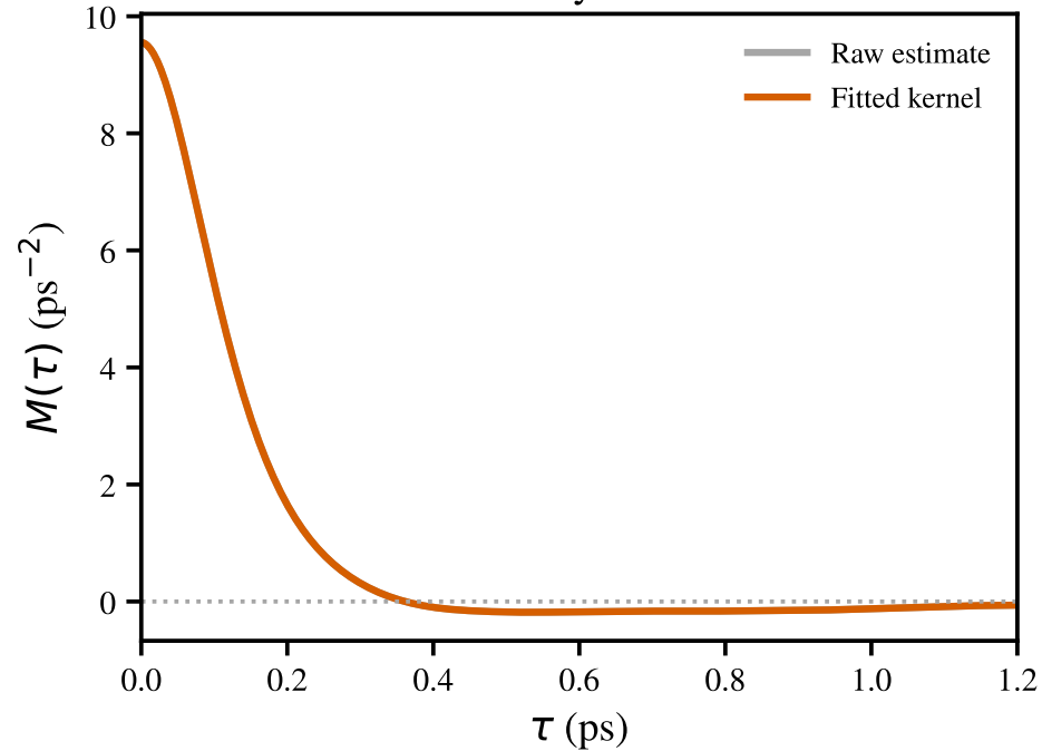
Memory kernel
