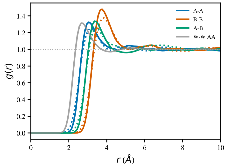
Bulk RDF
