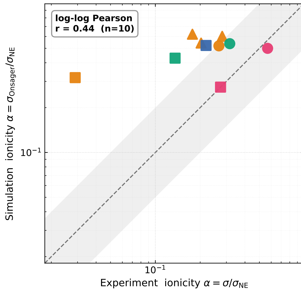
Ionicity (inverse Haven ratio) \alpha = \sigma/\sigma_{\text{NE}} : simulation vs experiment — \sigma_{\text{NE}} from Yeh-Hummer-corrected D (0.1 M excluded) PaiNN (FP32, NVT) OPLS-AA
