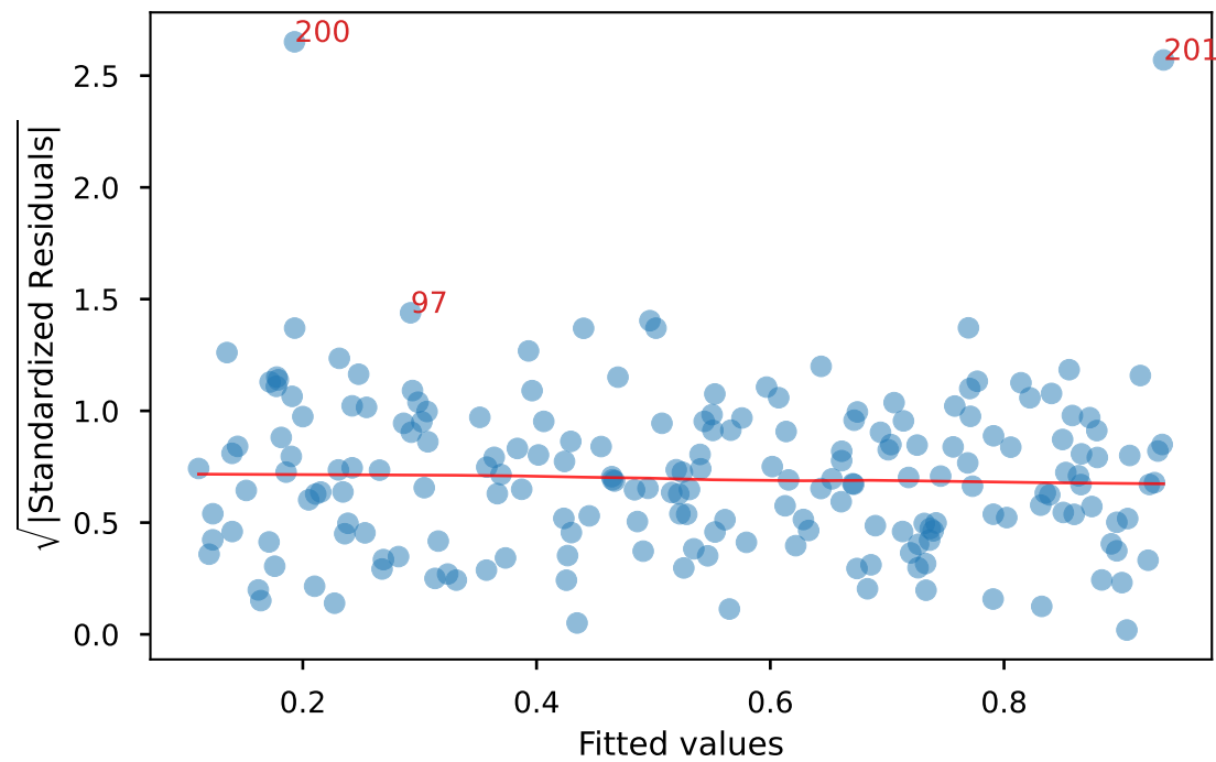
Scale-Location
