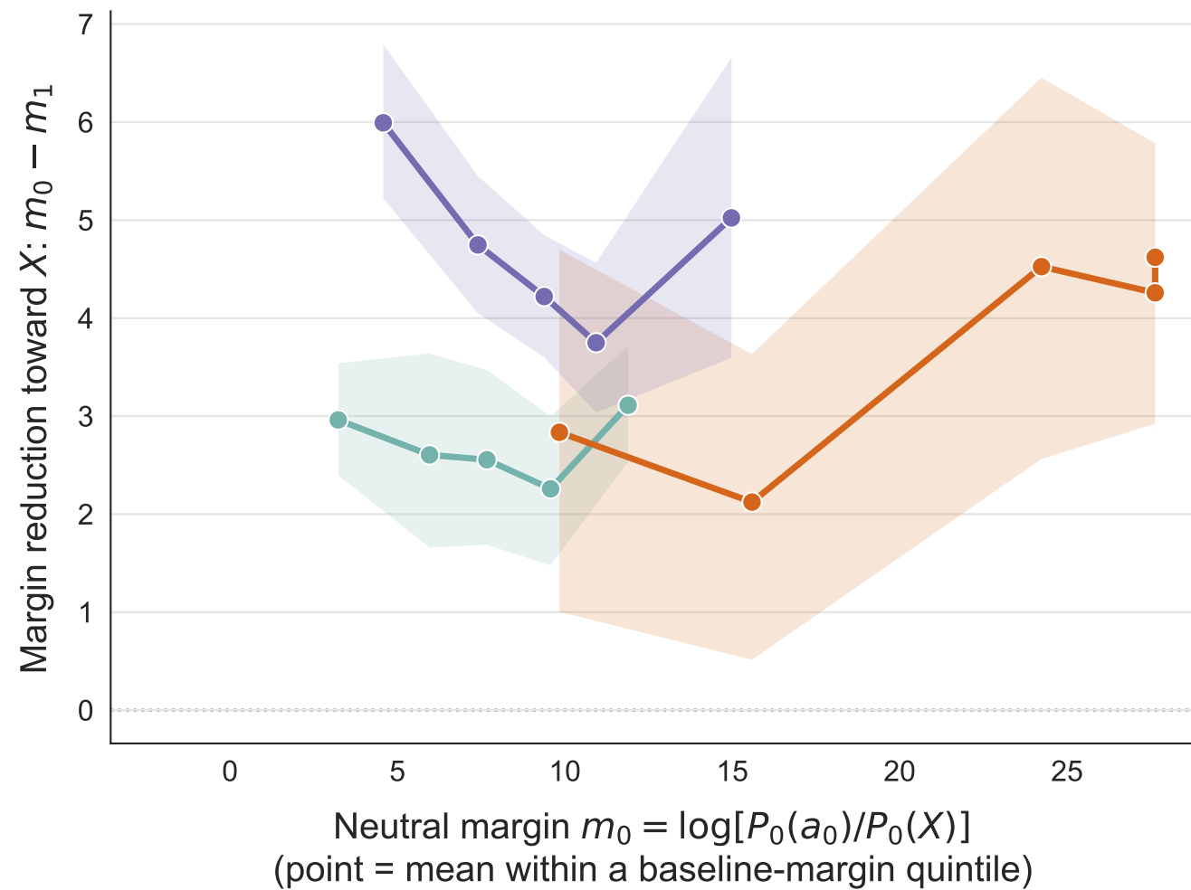
B. Endorsement-induced reduction in that margin
