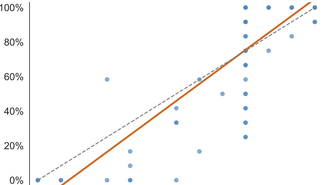
Claude Opus 5 Pearson r = 0.49 ; Spearman \rho = 0.45
