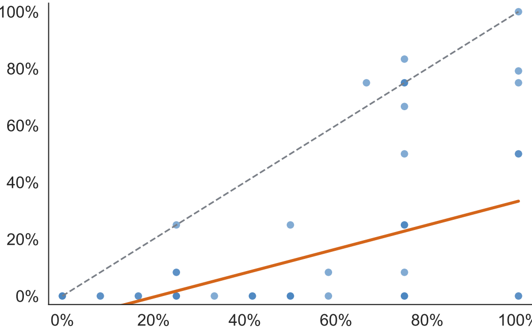
Claude Opus 5 Pearson r = 0.49 ; Spearman \rho = 0.45
