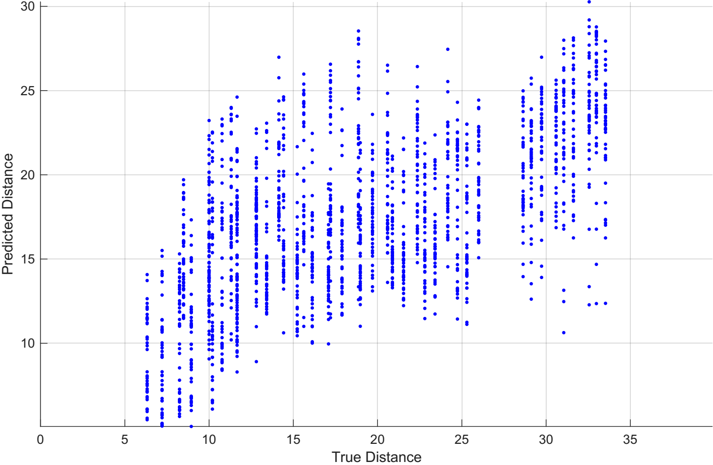
Random Forest: Split 1 (True vs Predicted)
