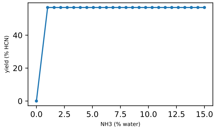
phenylalanine
