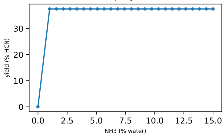
glutamine
