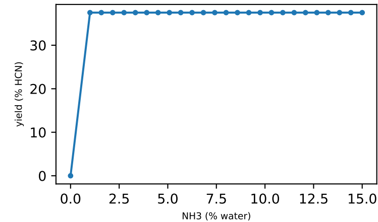
glycine
