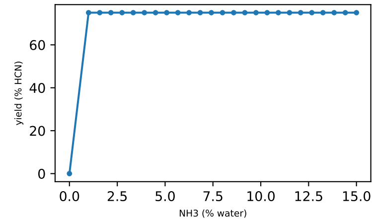
leucine
