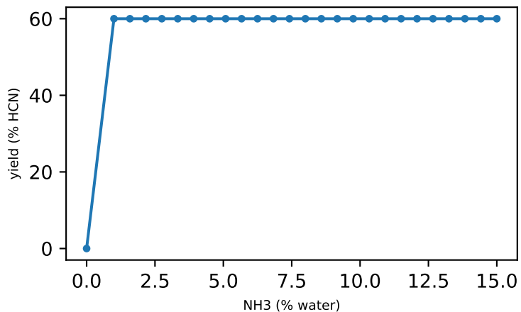
serine
