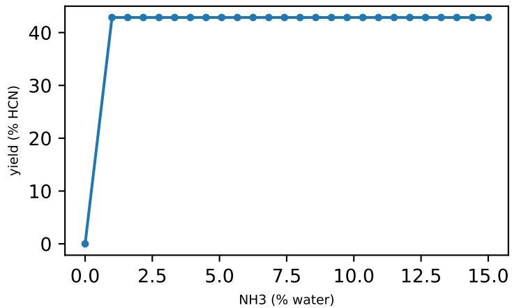
histidine
