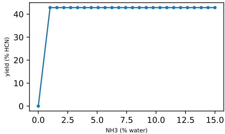
isoleucine
