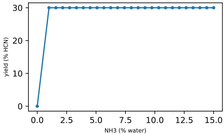
lysine
