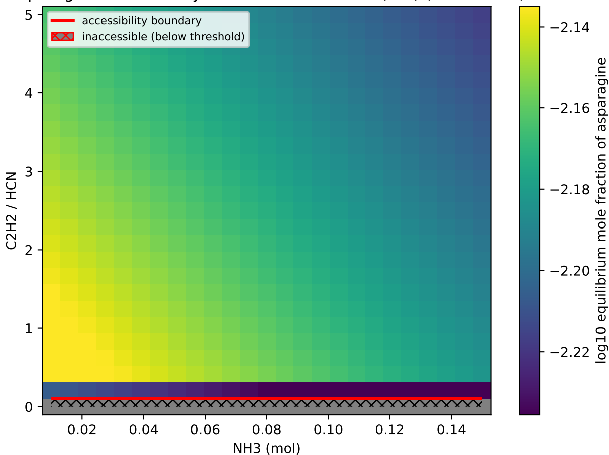
Asparagine accessibility — NH 3 vs C 2 H 2 /HCN (0 C) (autoscaled)
