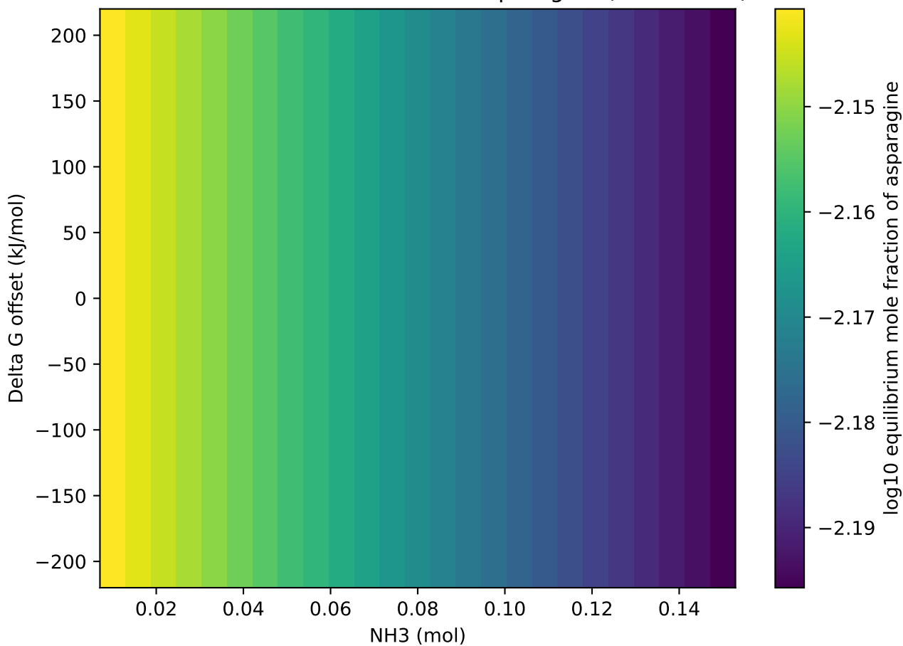
NH 3 threshold vs Gibbs offset for asparagine (autoscaled)
