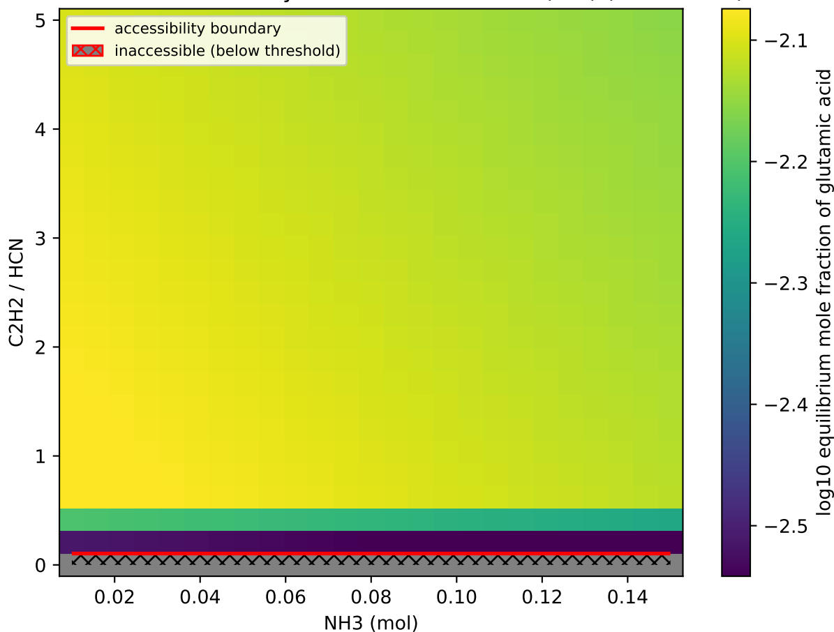
Glutamic Acid accessibility — \text{NH}_3 vs \text{C}_2\text{H}_2/\text{HCN} (0 C) (autoscaled)
