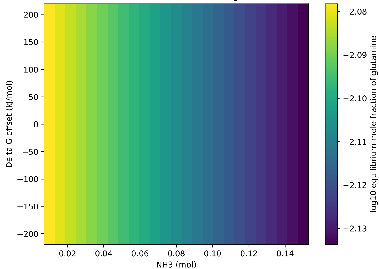
NH 3 threshold vs Gibbs offset for glutamine
