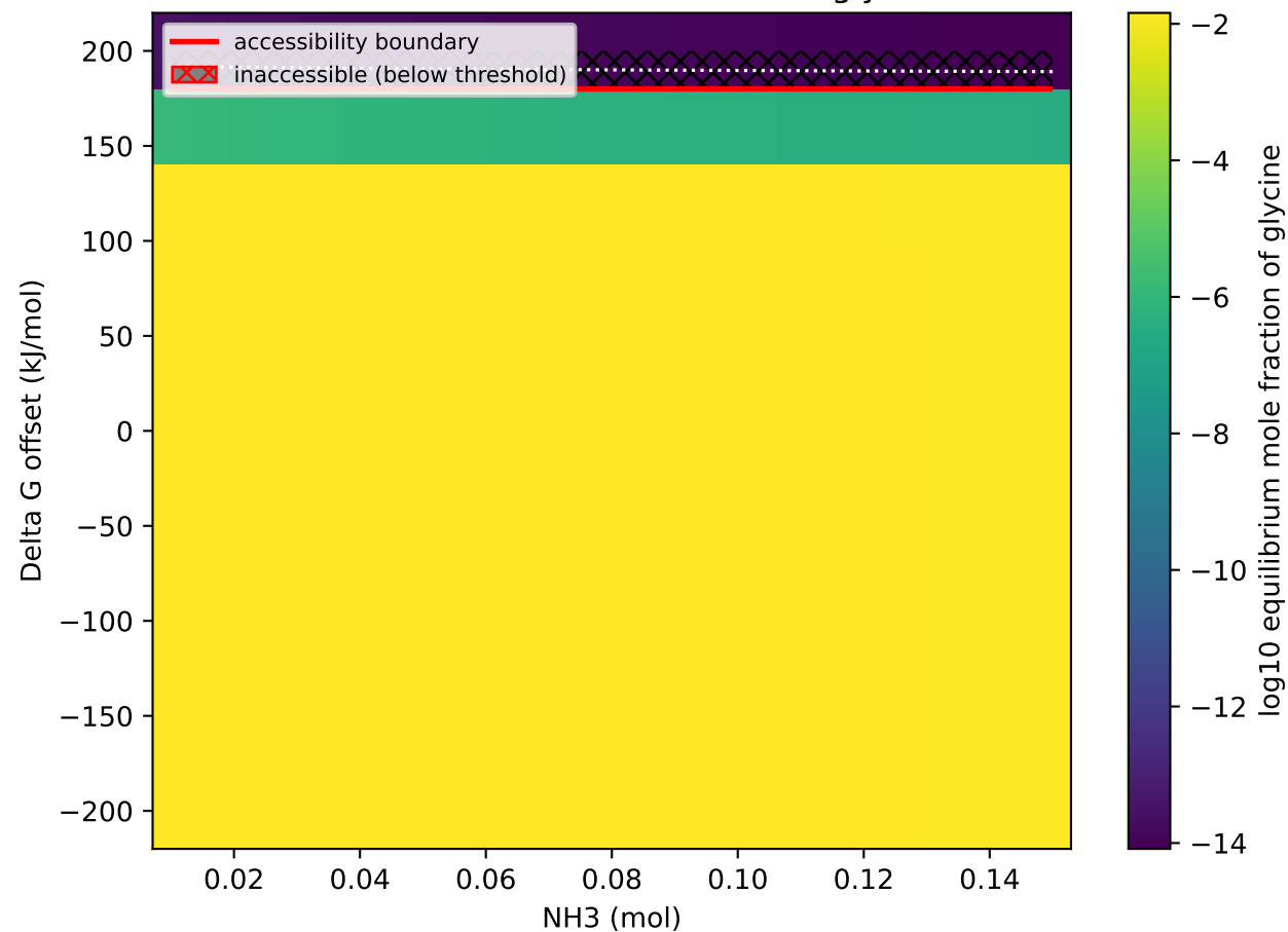
NH3 threshold vs Gibbs offset for glycine
