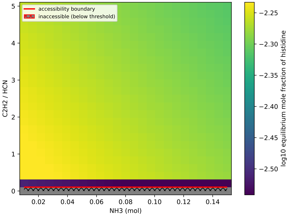
Histidine accessibility — NH3 vs C2H2/HCN (0 C) (autoscaled)
