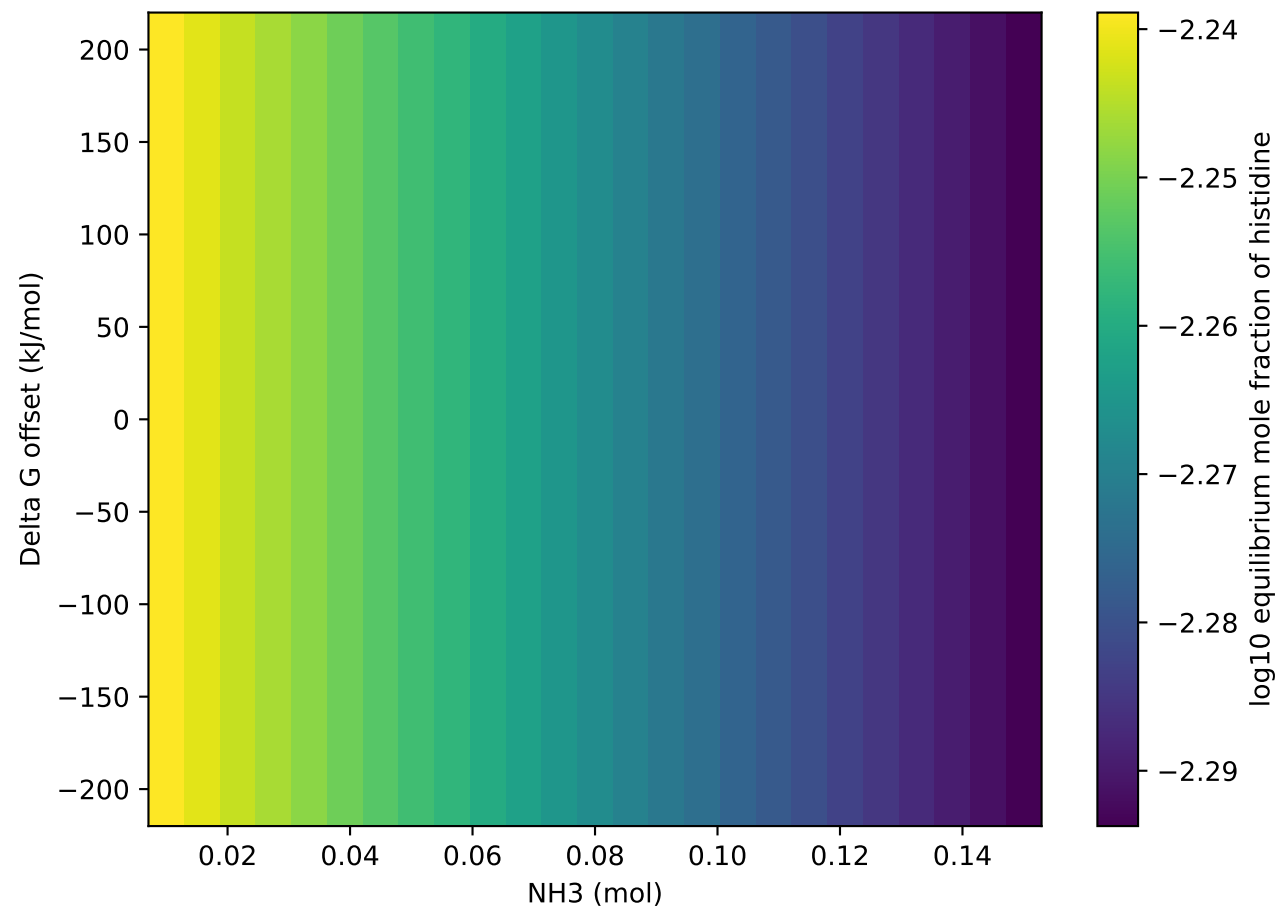
NH 3 threshold vs Gibbs offset for histidine
