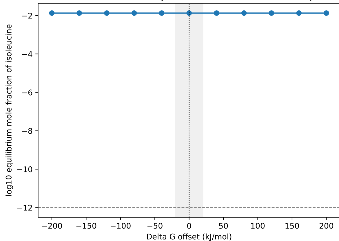
Isoleucine accessibility vs Gibbs offset (fixed inventory)
