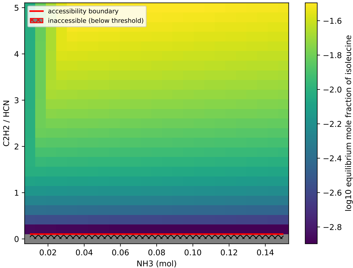
Isoleucine accessibility — NH 3 vs C 2 H 2 /HCN (0 C) (autoscaled)
