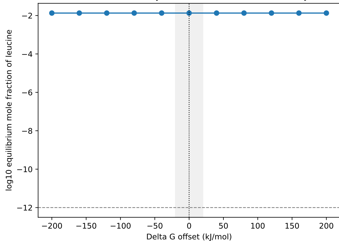
Leucine accessibility vs Gibbs offset (fixed inventory)
