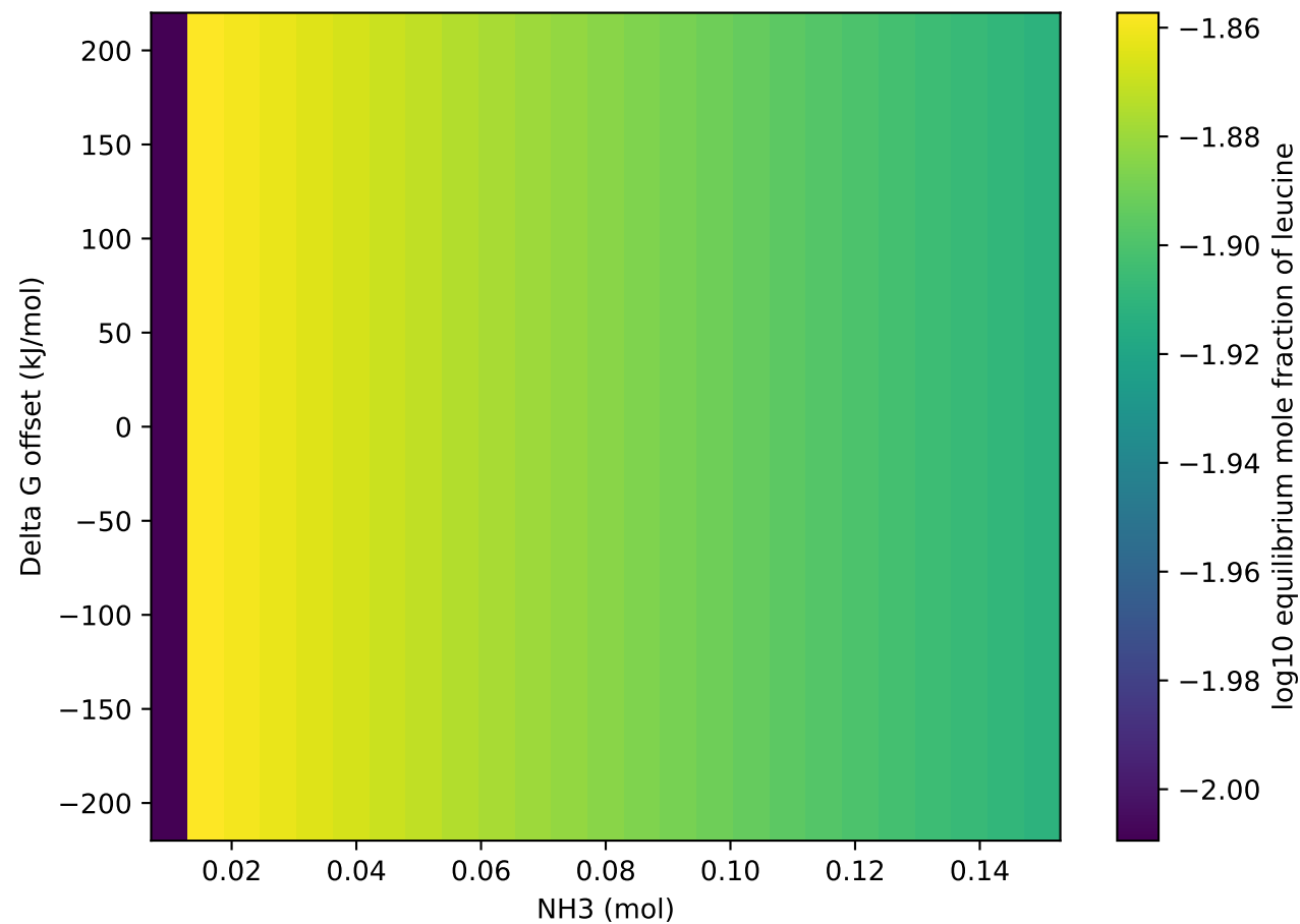
NH 3 threshold vs Gibbs offset for leucine
