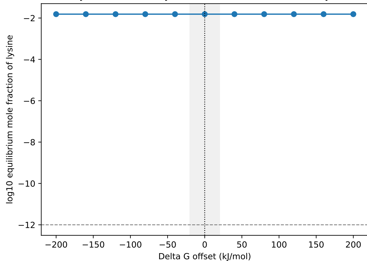
Lysine accessibility vs Gibbs offset (fixed inventory)
