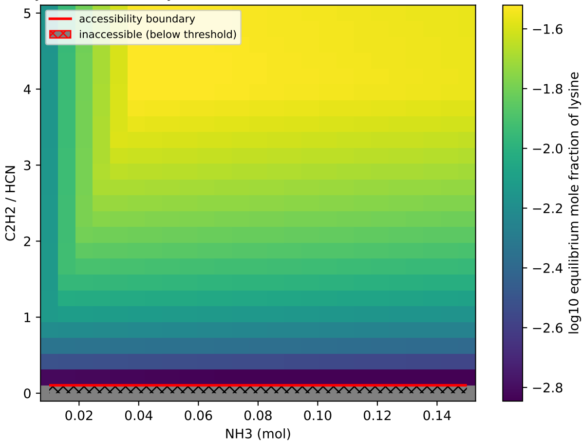
Lysine accessibility — NH 3 vs C 2 H 2 /HCN (0 C) (autoscaled)
