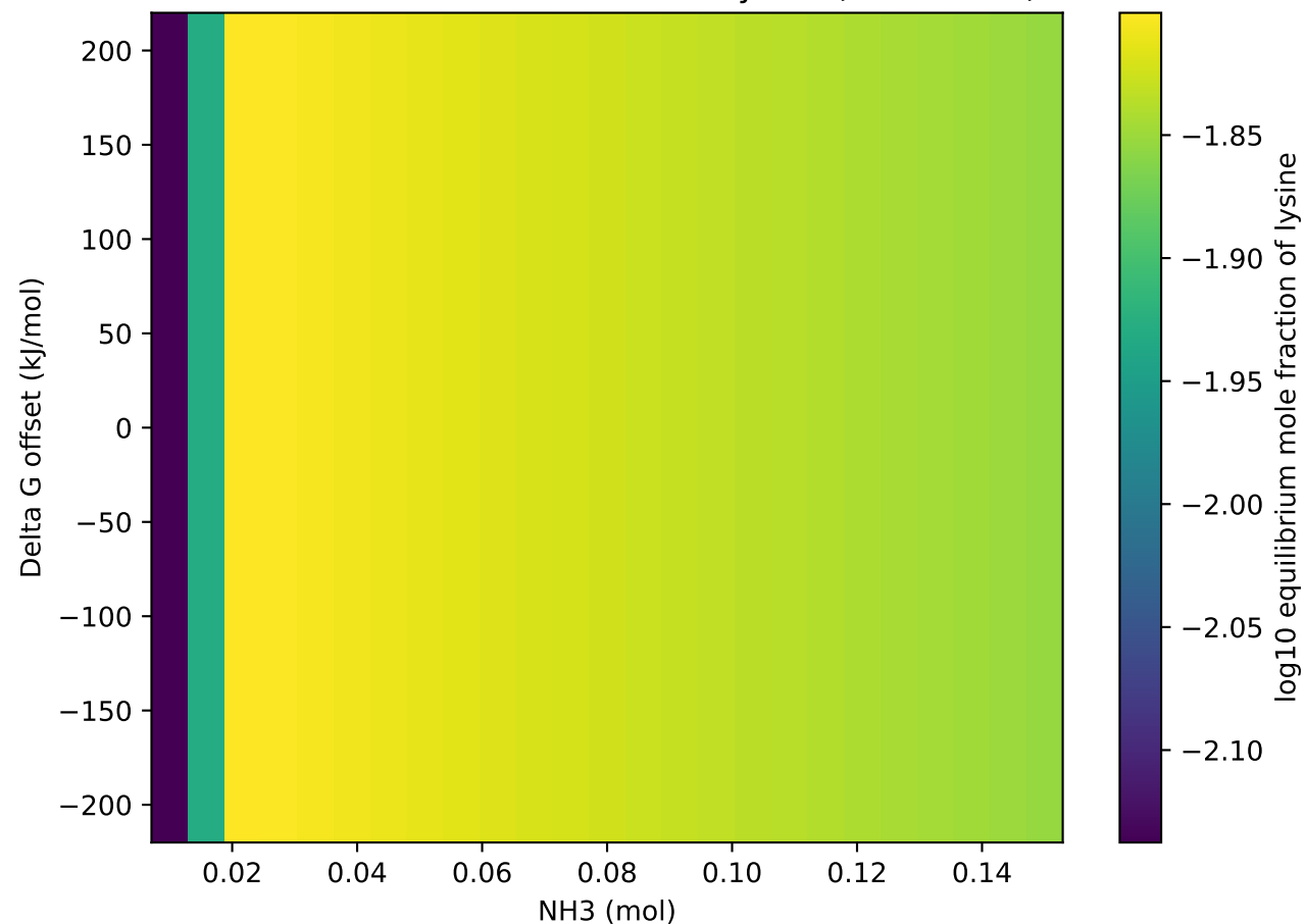
NH3 threshold vs Gibbs offset for lysine (autoscaled)
