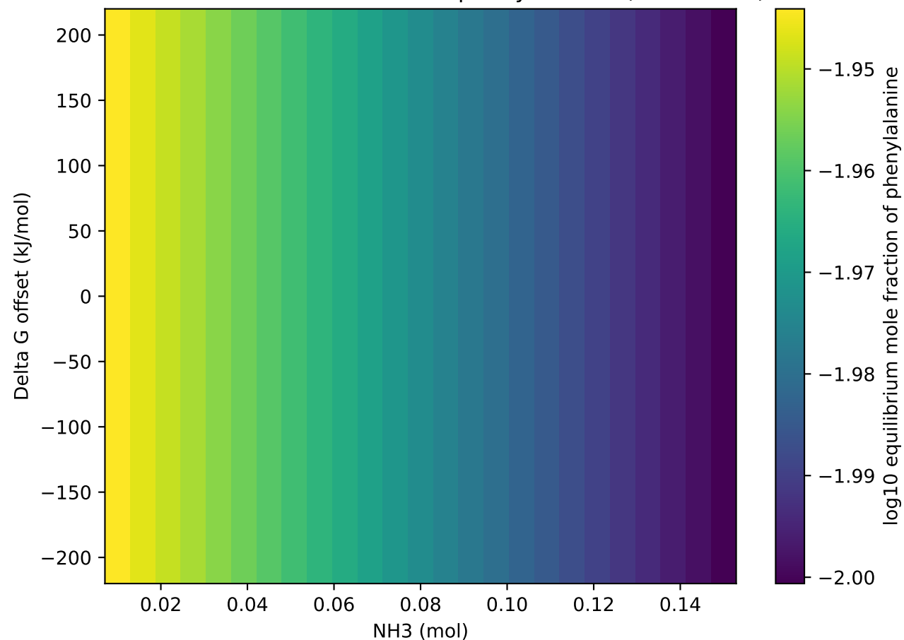
NH 3 threshold vs Gibbs offset for phenylalanine (autoscaled)
