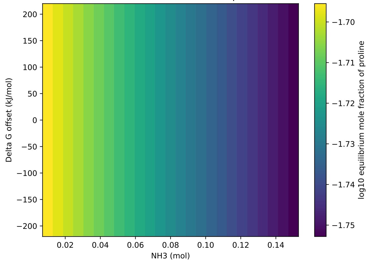
NH 3 threshold vs Gibbs offset for proline
