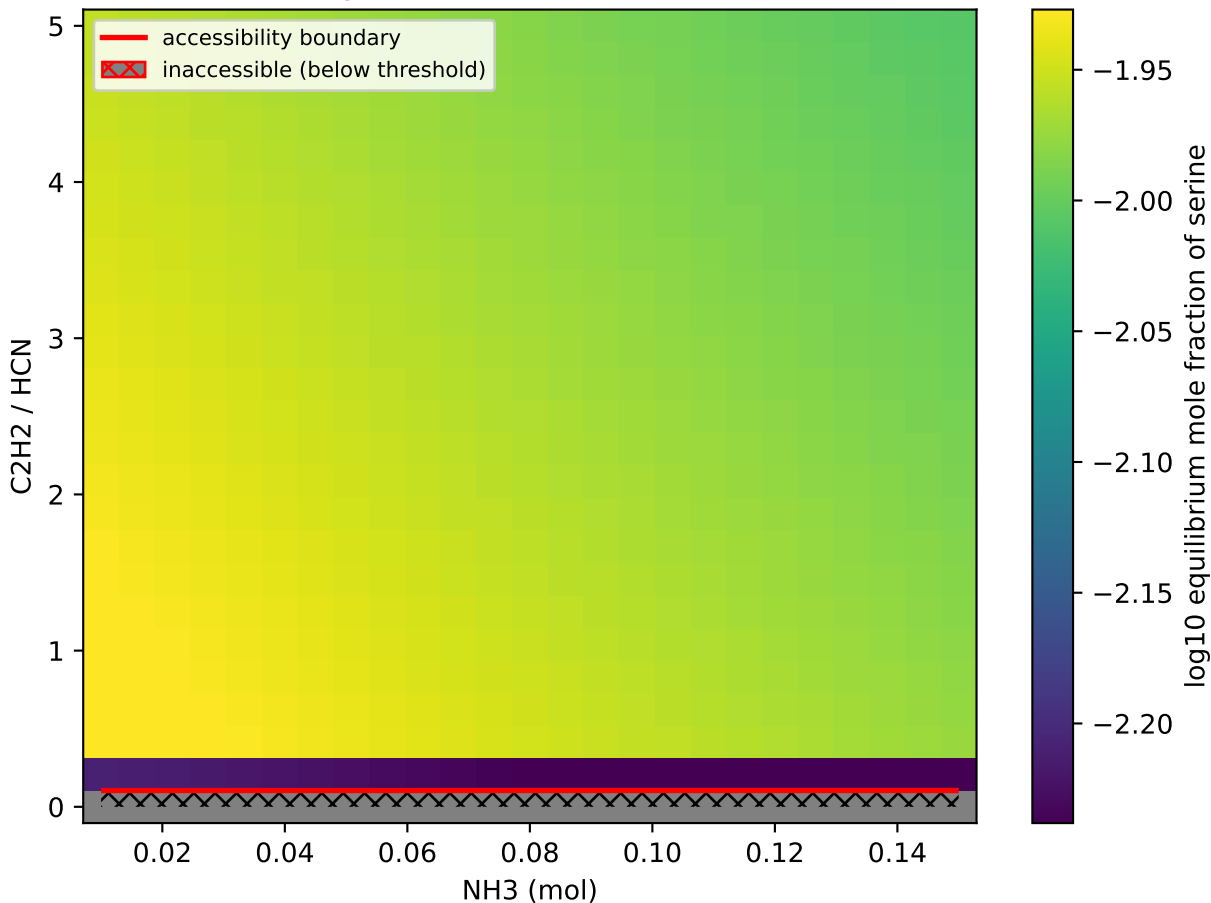
Serine accessibility — \text{NH}_3 vs \text{C}_2\text{H}_2/\text{HCN} (0 C) (autoscaled)
