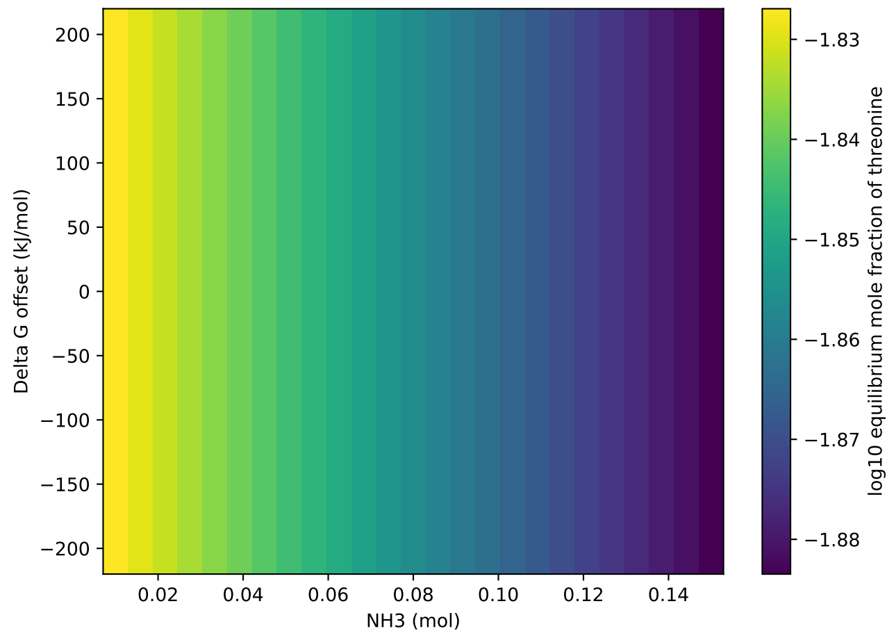
NH 3 threshold vs Gibbs offset for threonine
