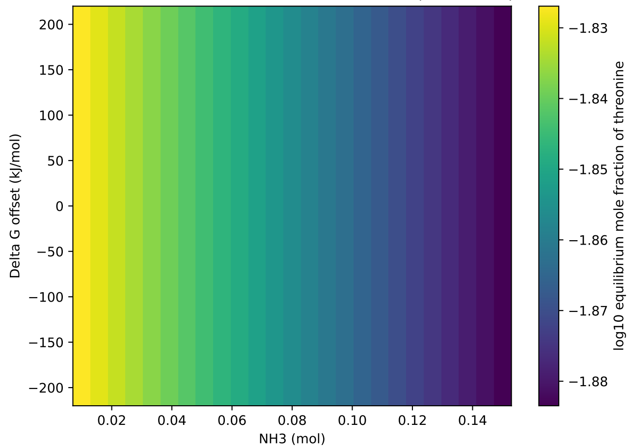
NH 3 threshold vs Gibbs offset for threonine (autoscaled)
