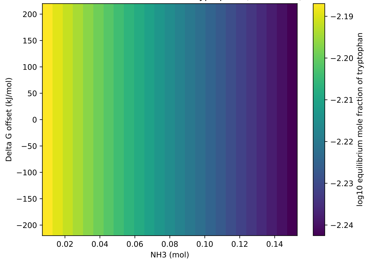
NH 3 threshold vs Gibbs offset for tryptophan (autoscaled)
