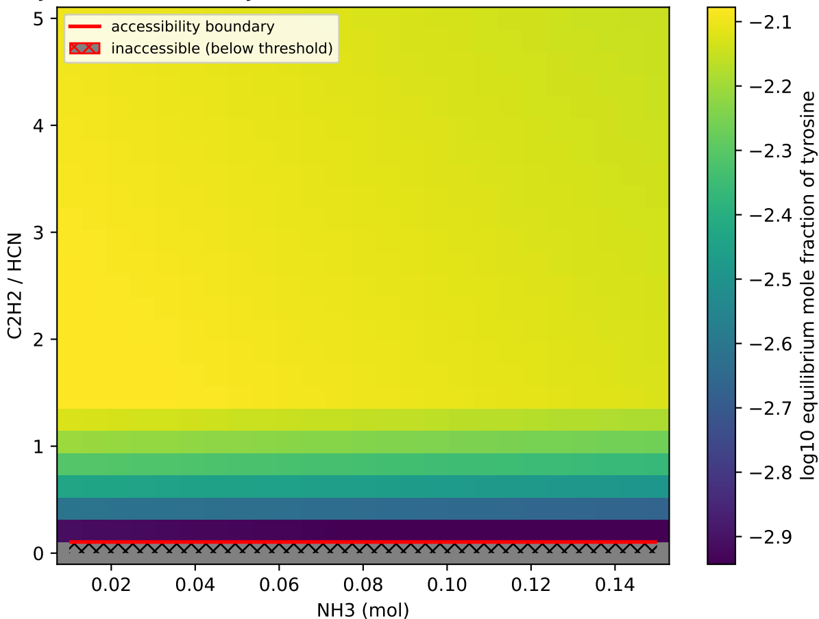
Tyrosine accessibility — NH 3 vs C 2 H 2 /HCN (0 C) (autoscaled)
