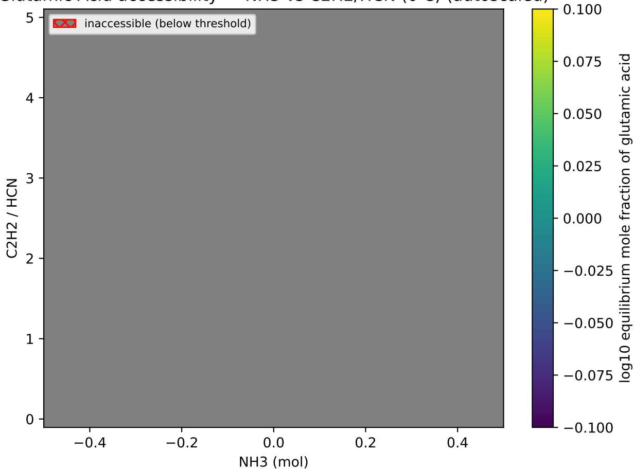
Glutamic Acid accessibility — NH3 vs C2H2/HCN (0 C) (autoscaled)
