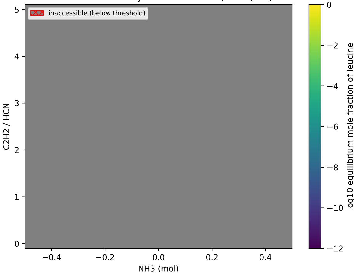
Leucine accessibility — NH 3 vs C 2 H 2 /HCN (0 C)
