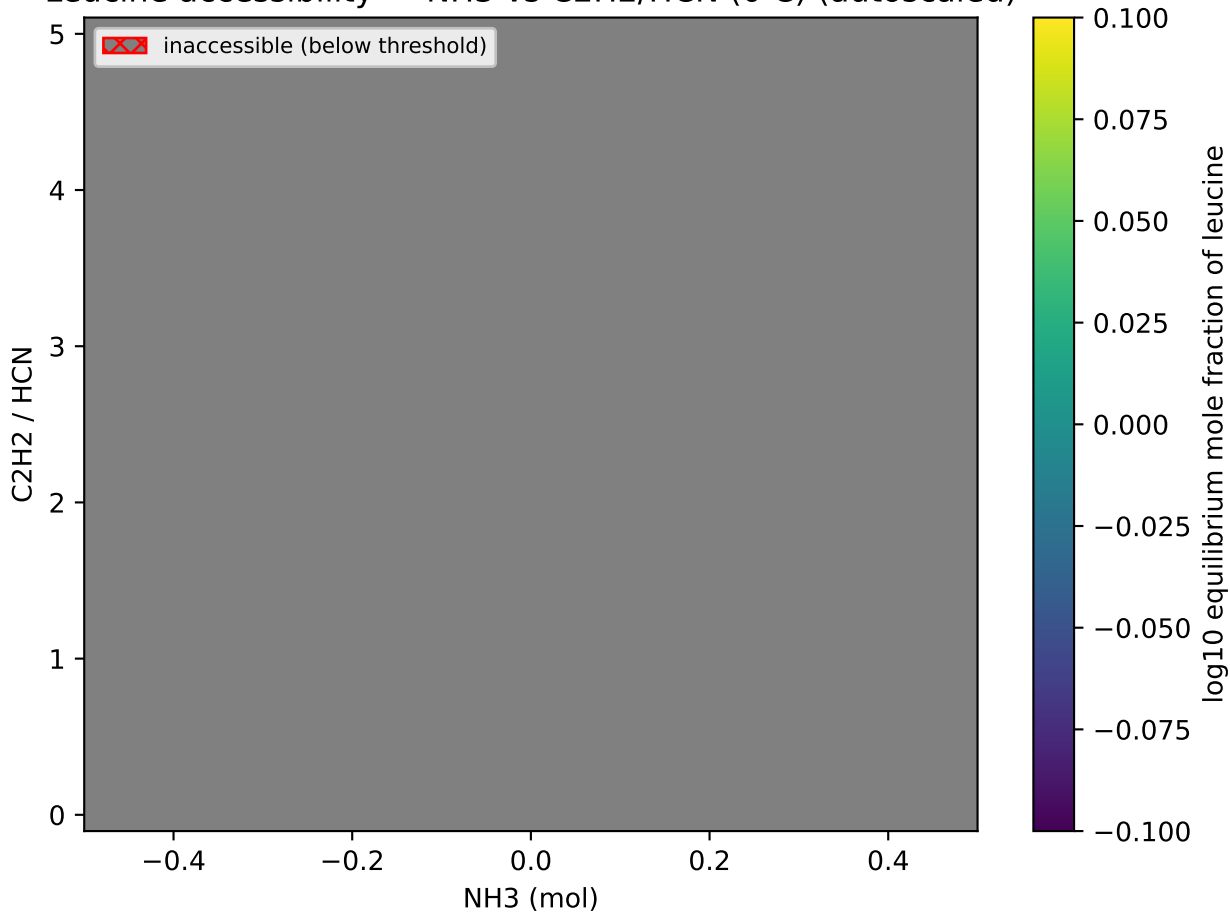
Leucine accessibility — NH 3 vs C 2 H 2 /HCN (0 C) (autoscaled)
