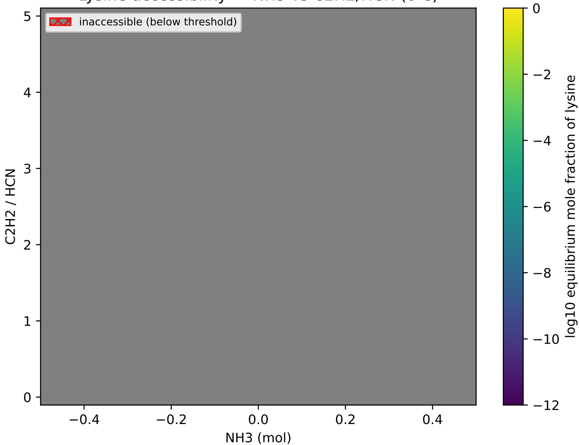
Lysine accessibility — NH3 vs C2H2/HCN (0 C)
