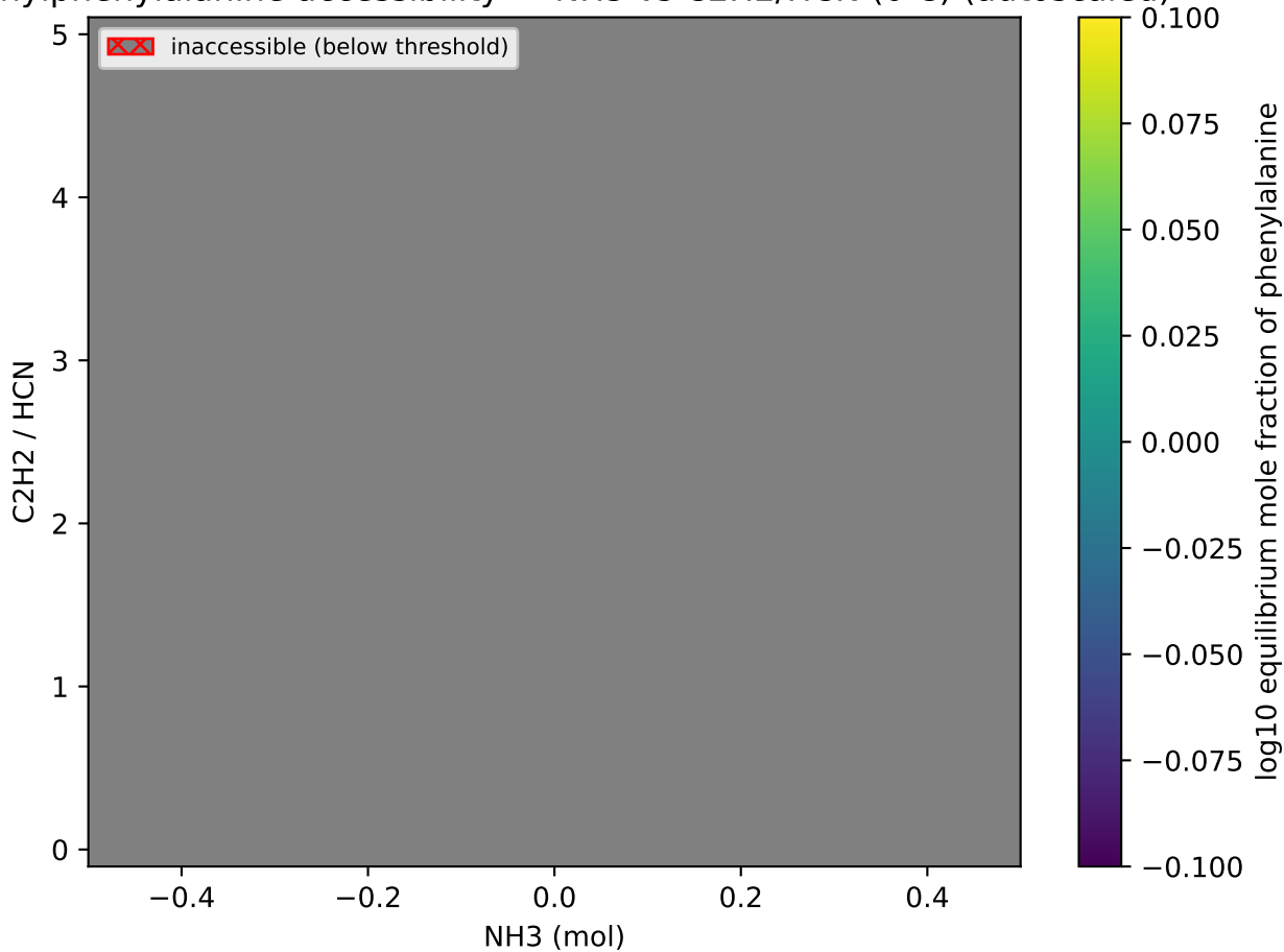
Phenylphenylalanine accessibility — NH3 vs C2H2/HCN (0 C) (autoscaled)
