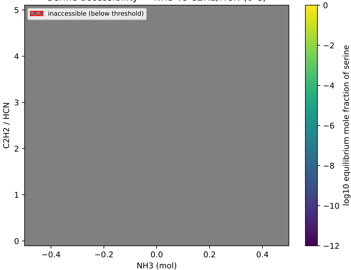
Serine accessibility — NH 3 vs C 2 H 2 /HCN (0 C)
