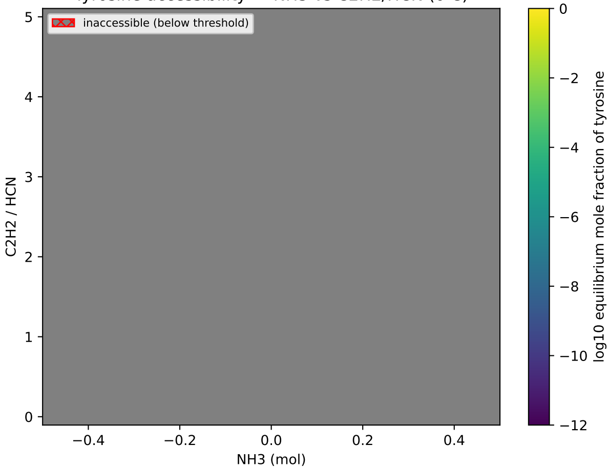
Tyrosine accessibility — NH 3 vs C 2 H 2 /HCN (0 C)
