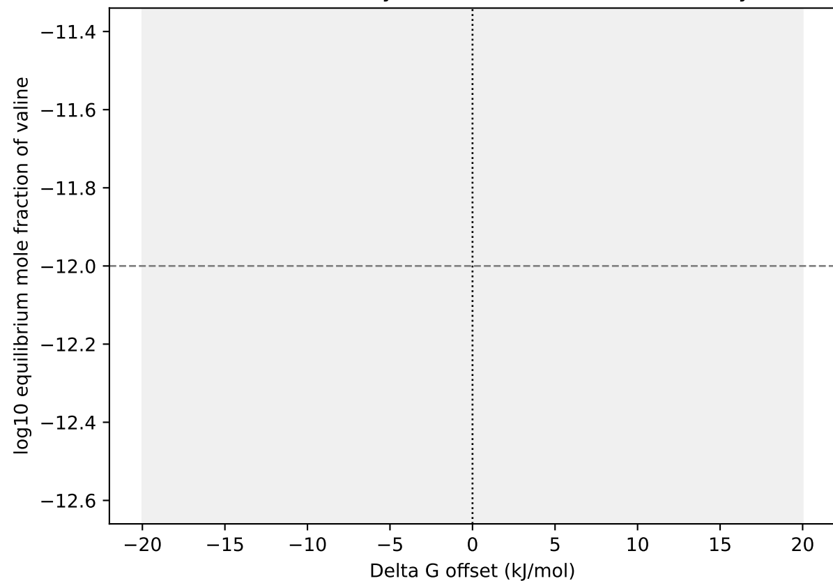
Valine accessibility vs Gibbs offset (fixed inventory)
