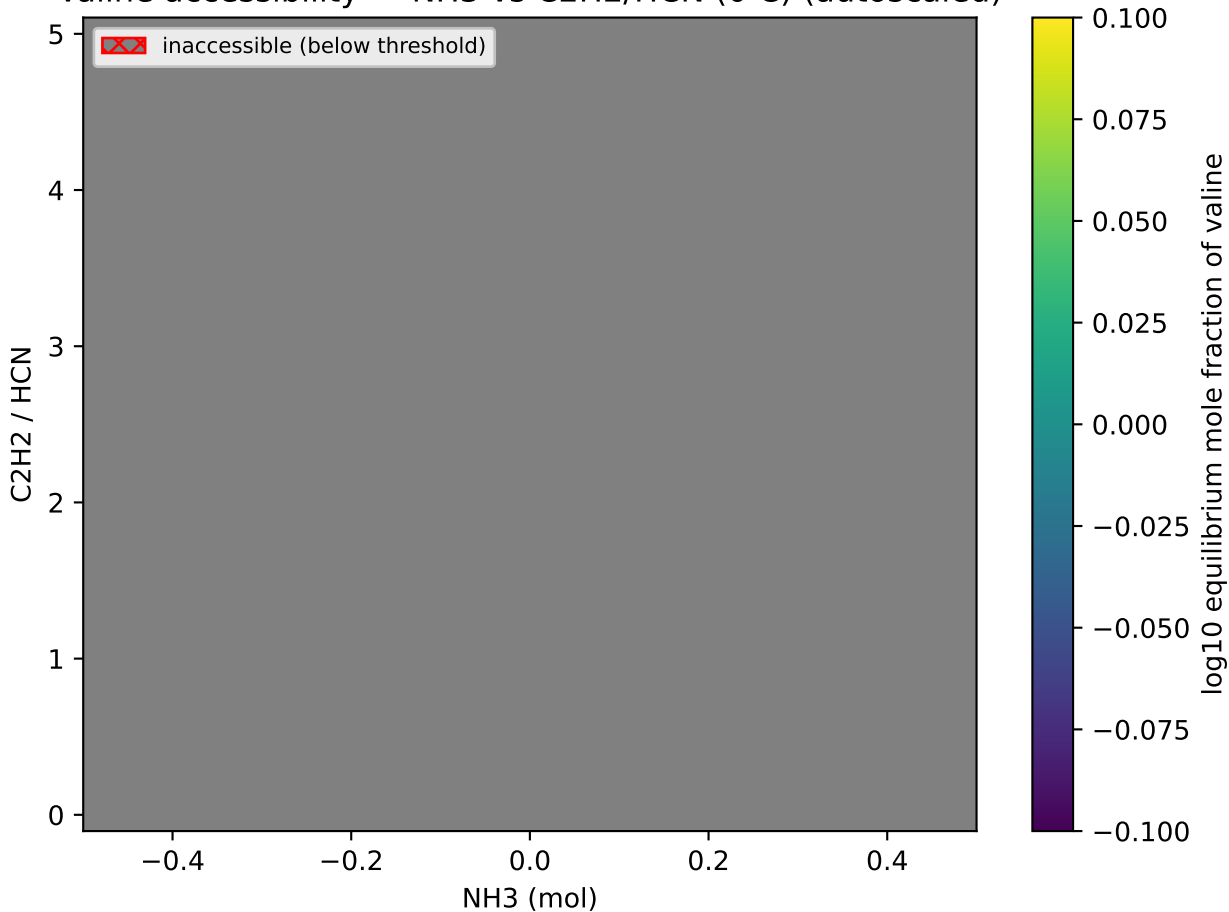
Valine accessibility — NH3 vs C2H2/HCN (0 C) (autoscaled)
