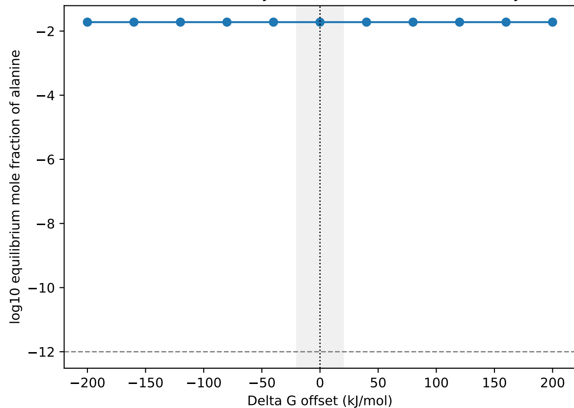
Alanine accessibility vs Gibbs offset (fixed inventory)
