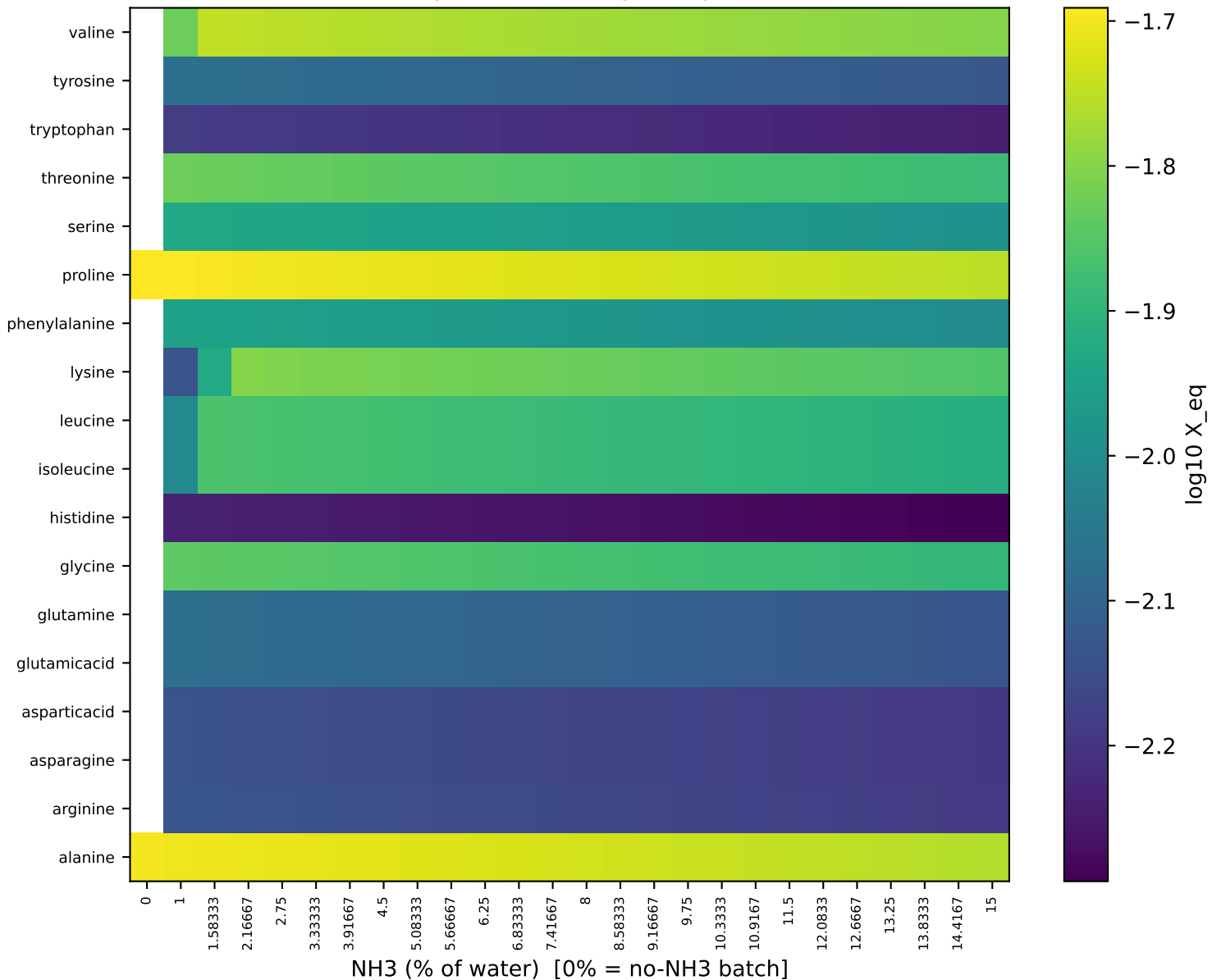
Amino-acid accessibility vs NH3 — log10 equilibrium mole fraction
