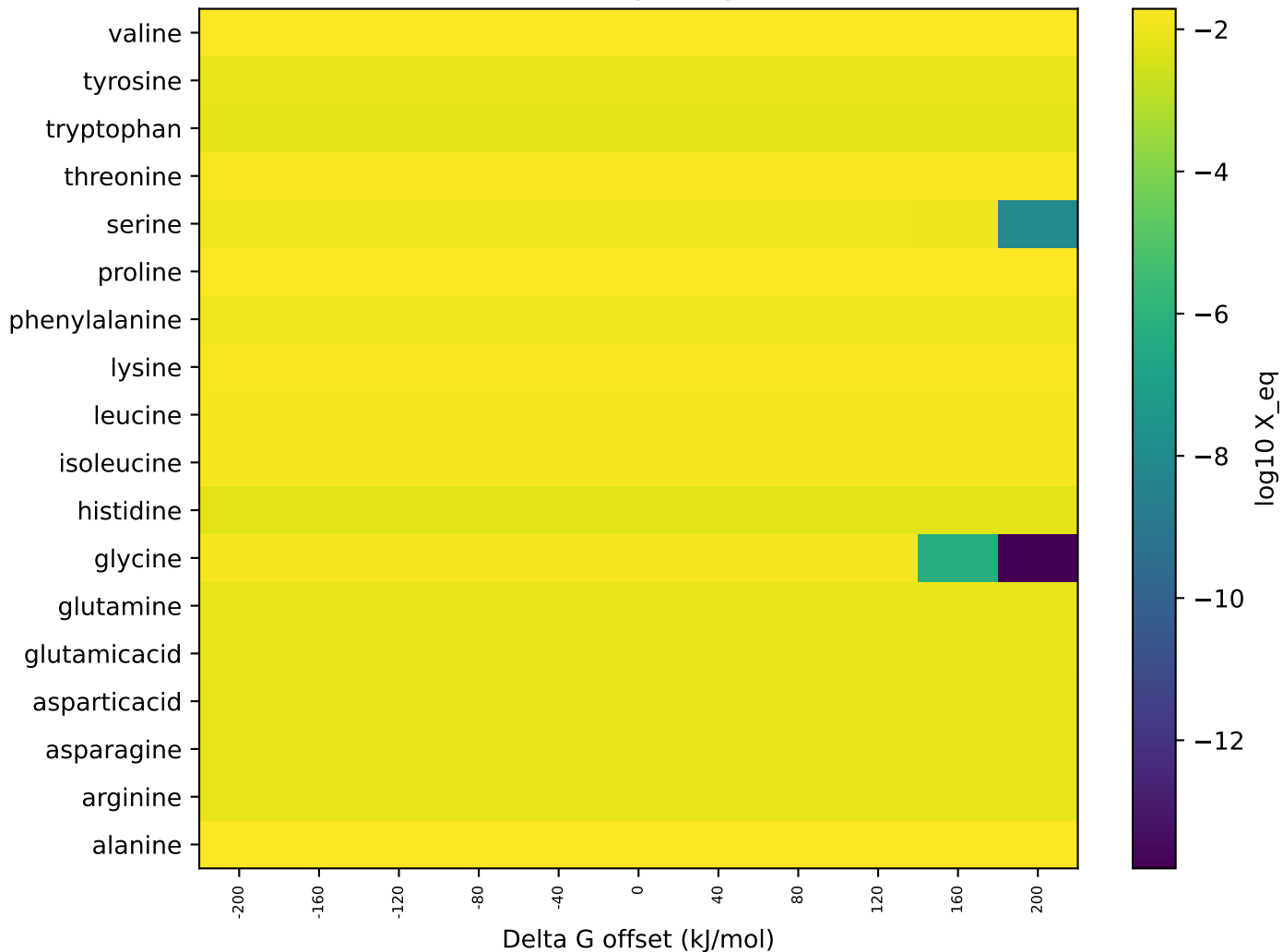
Amino acid \times \Delta G offset — \log_{10} equilibrium mole fraction
