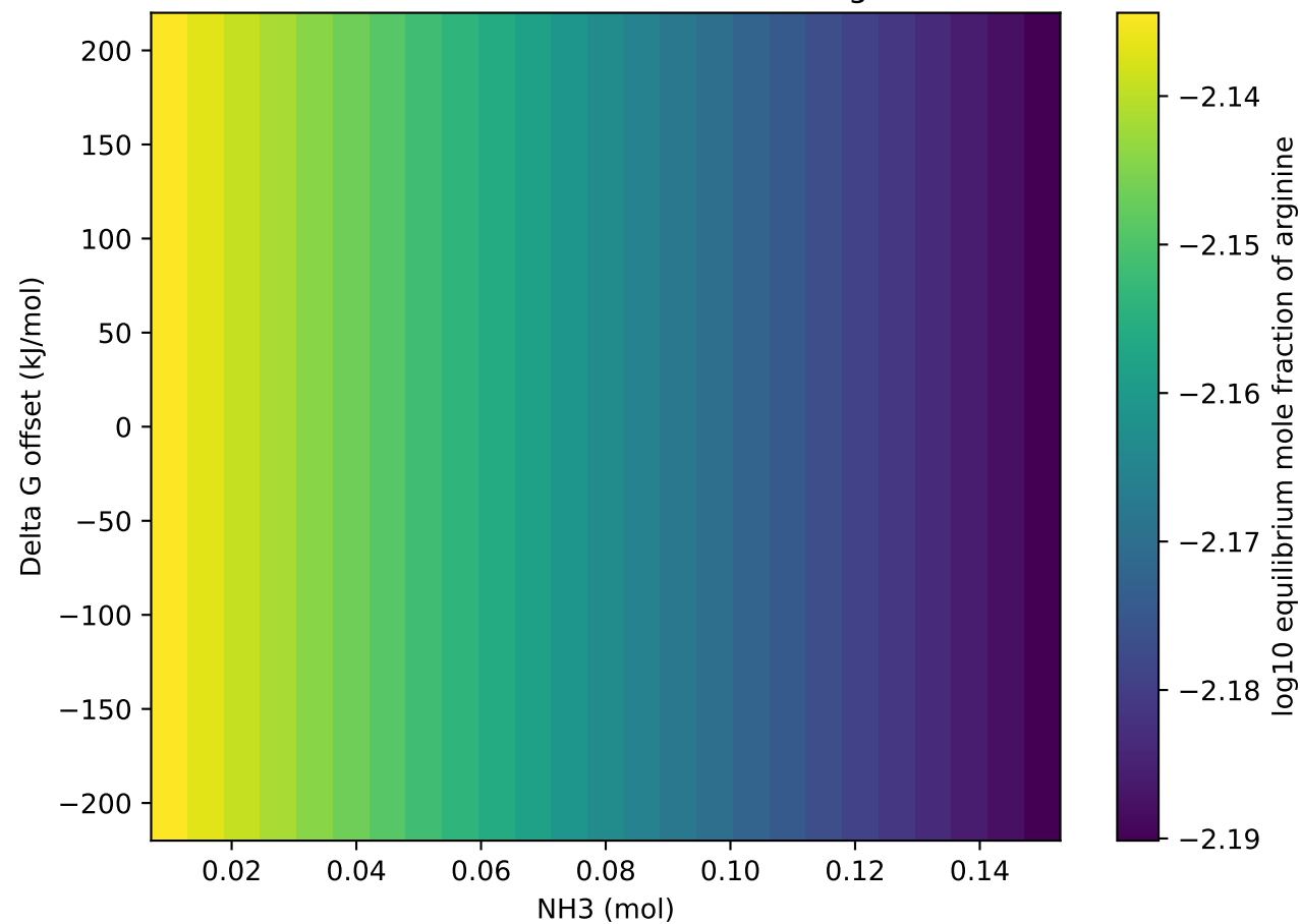
NH 3 threshold vs Gibbs offset for arginine
