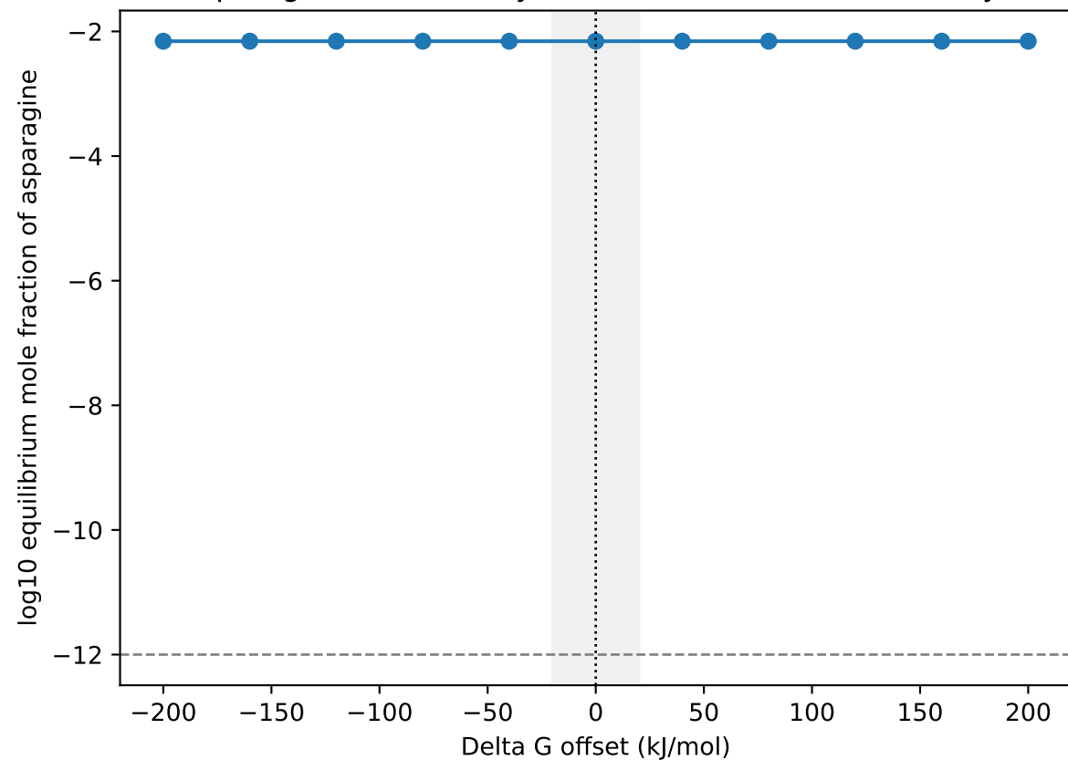
Asparagine accessibility vs Gibbs offset (fixed inventory)
