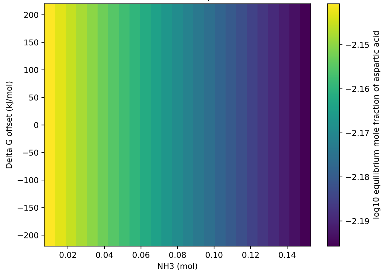
NH 3 threshold vs Gibbs offset for aspartic acid (autoscaled)
