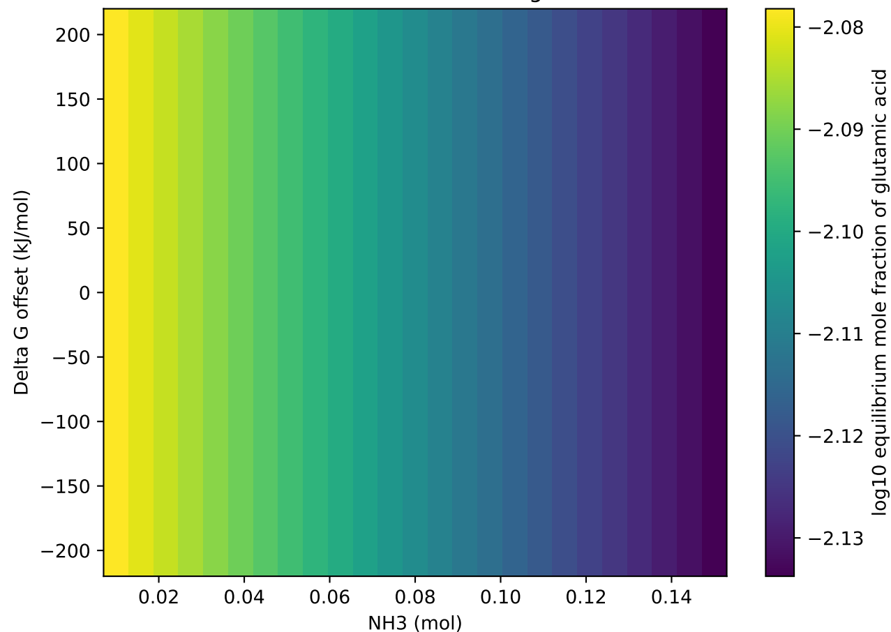
NH 3 threshold vs Gibbs offset for glutamic acid
