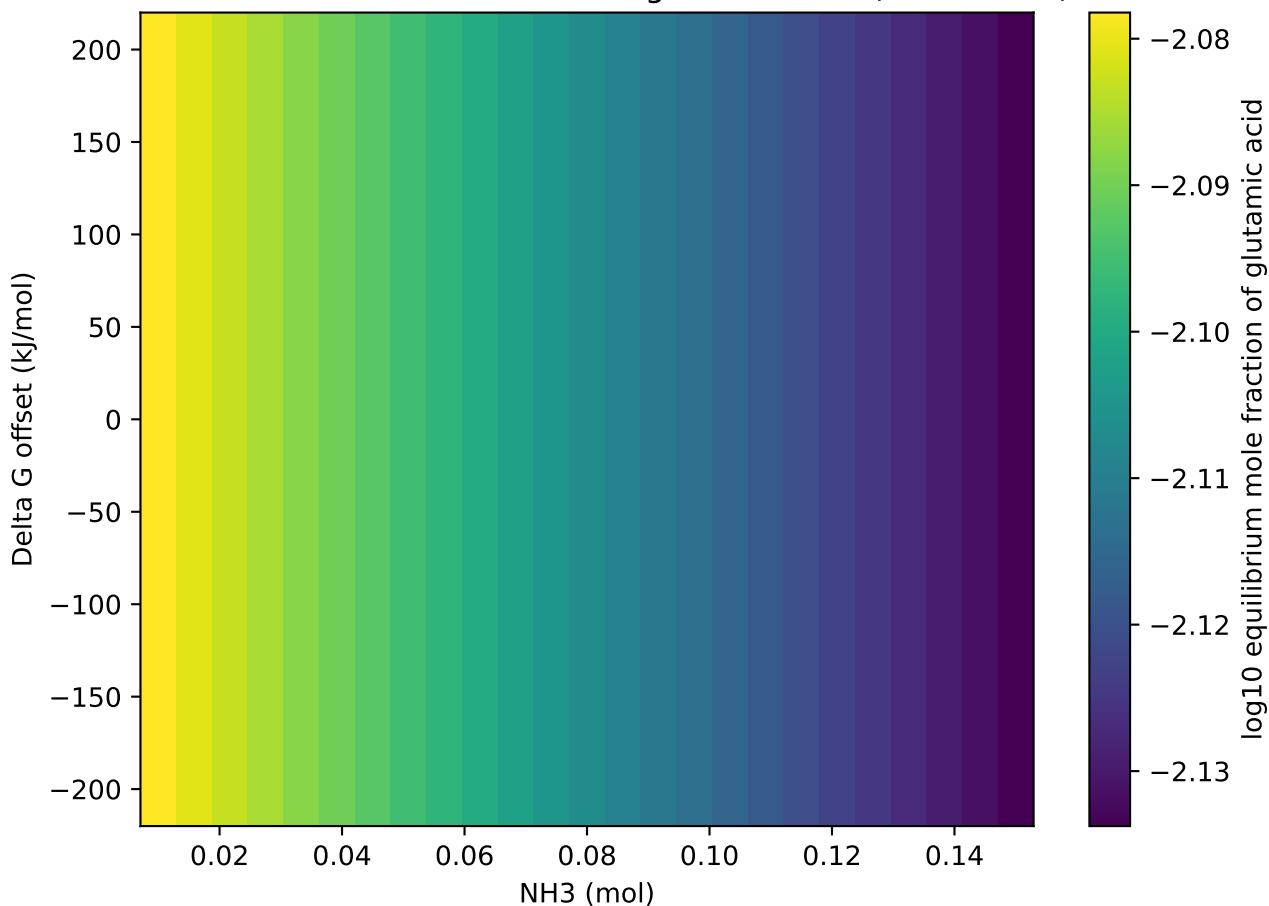
NH 3 threshold vs Gibbs offset for glutamic acid (autoscaled)
