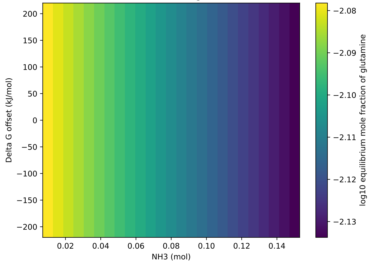
NH 3 threshold vs Gibbs offset for glutamine (autoscaled)
